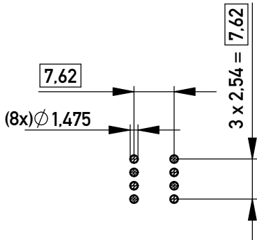
Layout - Vorschlag PCB - Layout proposal M / scale 2:1
