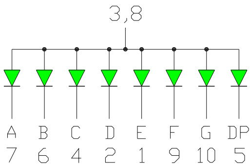
SMA201SPG-UT G/W ( Common Anode )
