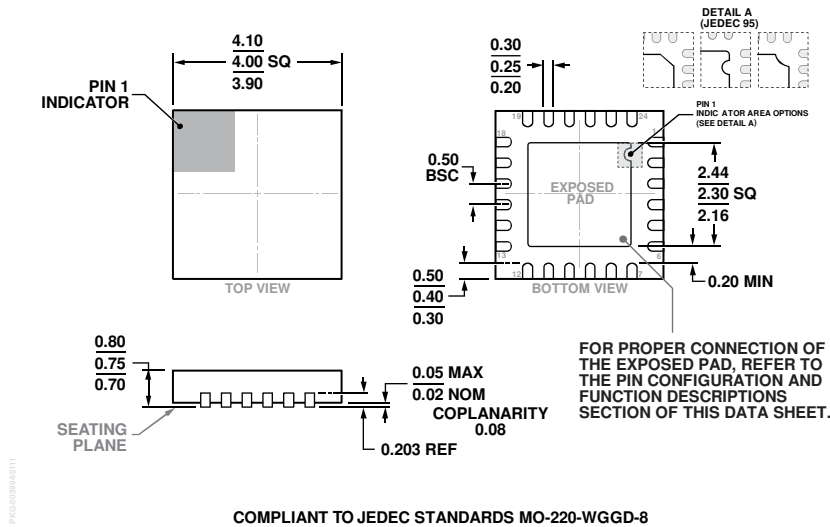
COMPLIANT TO JEDEC STANDARDS MO-220-WGGD-8 Figure 61. 24-Lead Lead Frame Chip Scale Package [LFCSP] 4 mm × 4 mm Body and 0.75 mm Package Height (CP-24-14) Dimensions shown in millimeters
