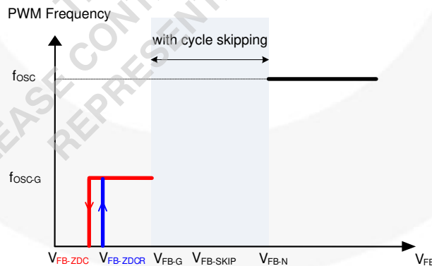
Figure 5. PWM Frequency
