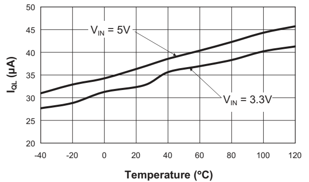
Quiescent Current I_{QL} vs. Temperature ( ENLB = 0V ; ENUB = V_{CC} ; V_{OUT} = \text{Open} )
