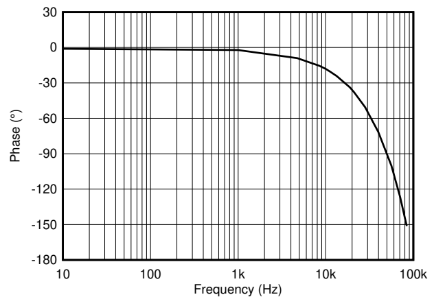
Figure 9-10. Normalized Phase, All Variants
