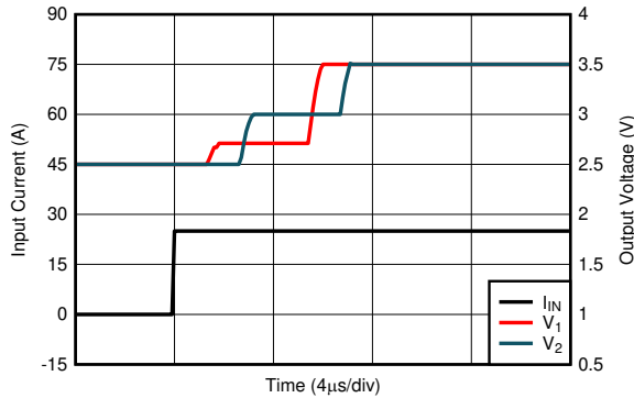
Figure 7-23. Voltage Output Step, Rising
