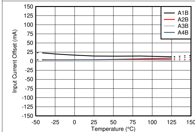
Figure 7-3. TMCS1101AxB-Q1 Input Offset Current vs Temperature
