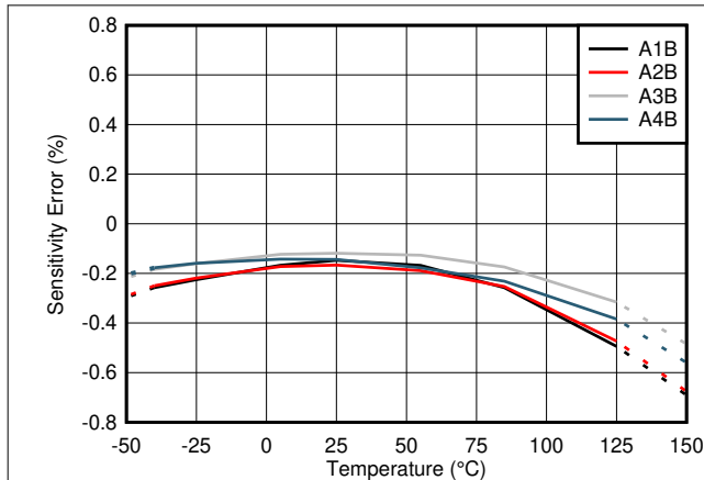
Figure 7-1. TMCS1101AxB-Q1 Sensitivity Error vs Temperature
