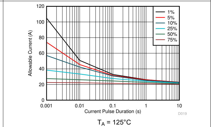
Figure 8-9. Maximum Repetitive Pulsed Current vs. Pulse Duration
