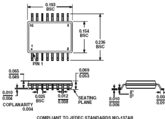
COMPLIANT TO JEDEC STANDARDS MO-137AB Figure 19. 16-Lead Shrink Small Outline Package [QSOP] (RQ-16) Dimensions shown in inches
