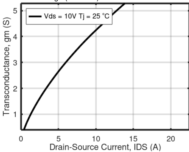
Figure 7: Transconductance vs. Drain Current For Room Temperature
