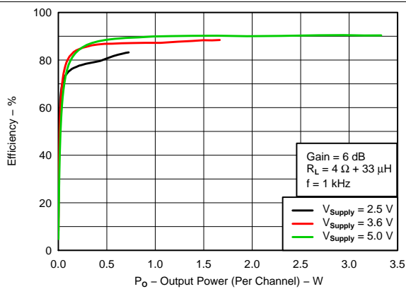
Figure 19. Efficiency vs Output Power (Per Channel), 4 Ω
