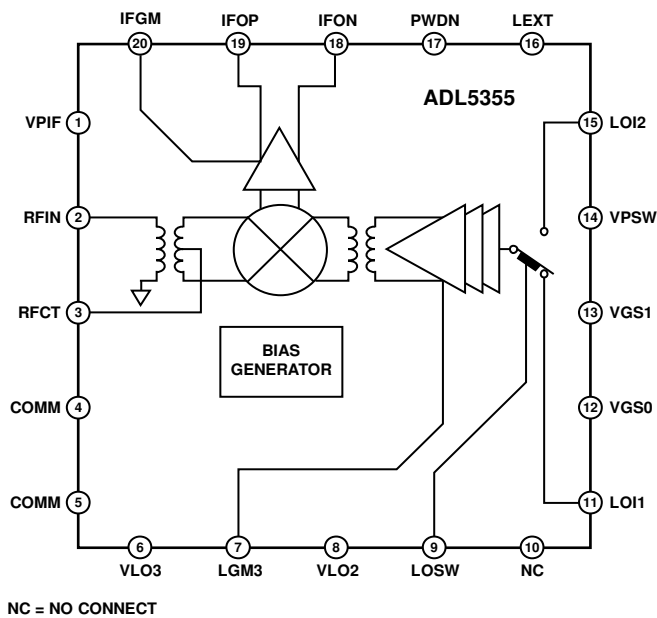
Figure 50. Simplified Schematic
