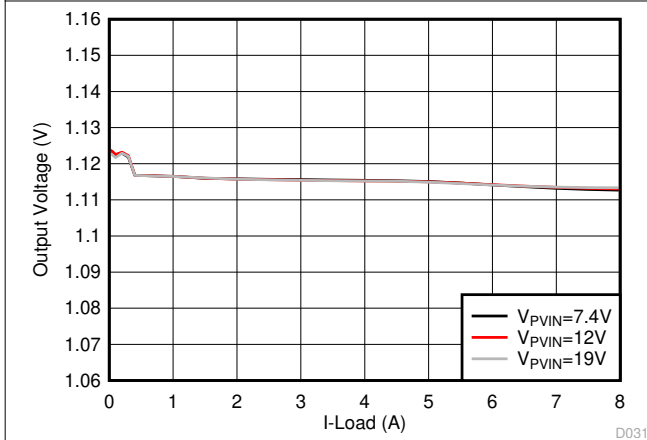
Figure 8-5. VDD2 Load Regulation, V_{OUT} = 1.1\text{ V}
