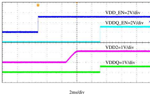
Figure 8-19. VDDQ Start-Up Through VDDQ_EN
