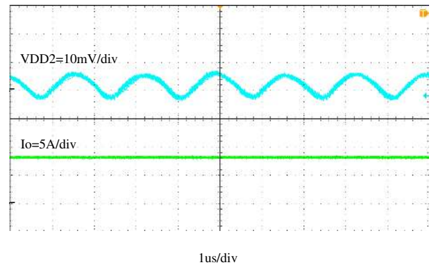
Figure 8-12. VDD2 Output Voltage Ripple, I_{OUT} = 8\text{ A}
