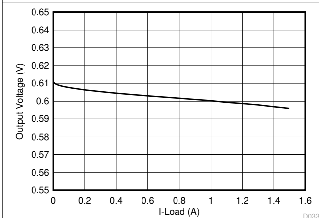
Figure 8-7. VDDQ Load Regulation, V_{OUT} = 0.6\text{ V}
