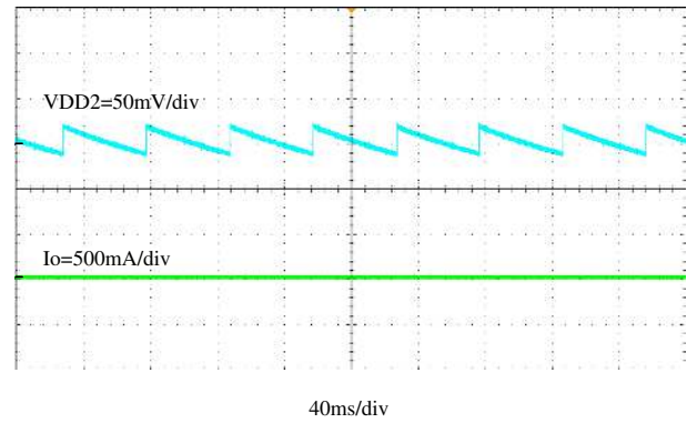
Figure 8-10. VDD2 Output Voltage Ripple, I_{OUT} = 0\text{ A}
