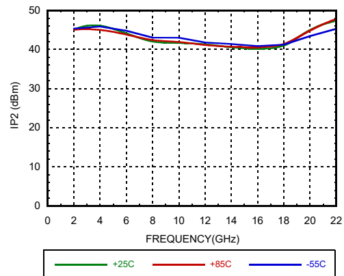
Output IP2 vs. Temperature @ Pout/Tone = +18 dBm
