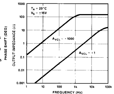
CLOSED-LOOP OUTPUT RESISTANCE vs FREQUENCY
