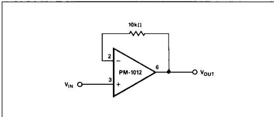
FIGURE 5: Unity-Gain Follower
