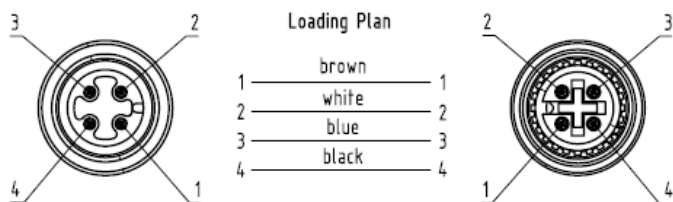
Male and Female 4-pole
