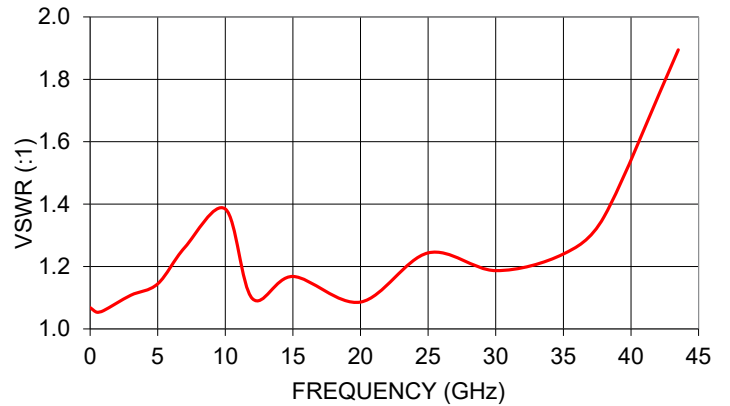
KAT-2+ VSWR
