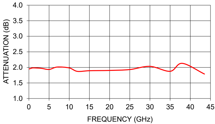
KAT-2+ ATTENUATION
