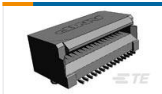
TE Part #788862-2 PT30 XFP CONNECTOR
