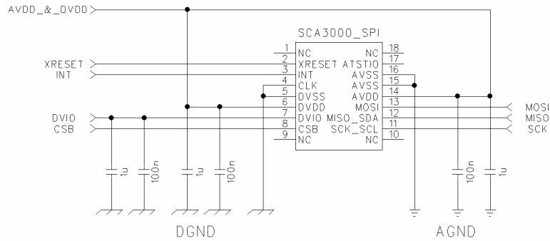
Figure 6 Application schematic
