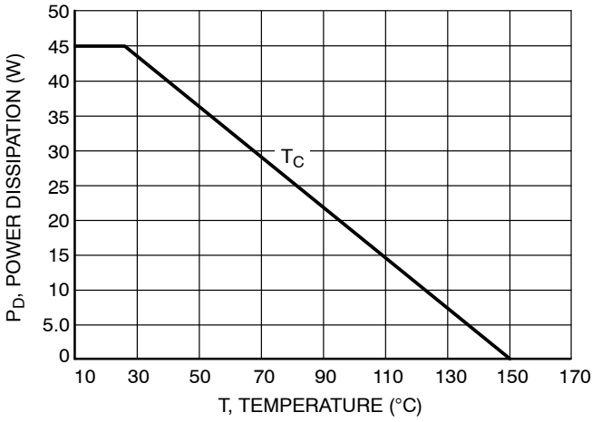
Figure 2. Power Derating
