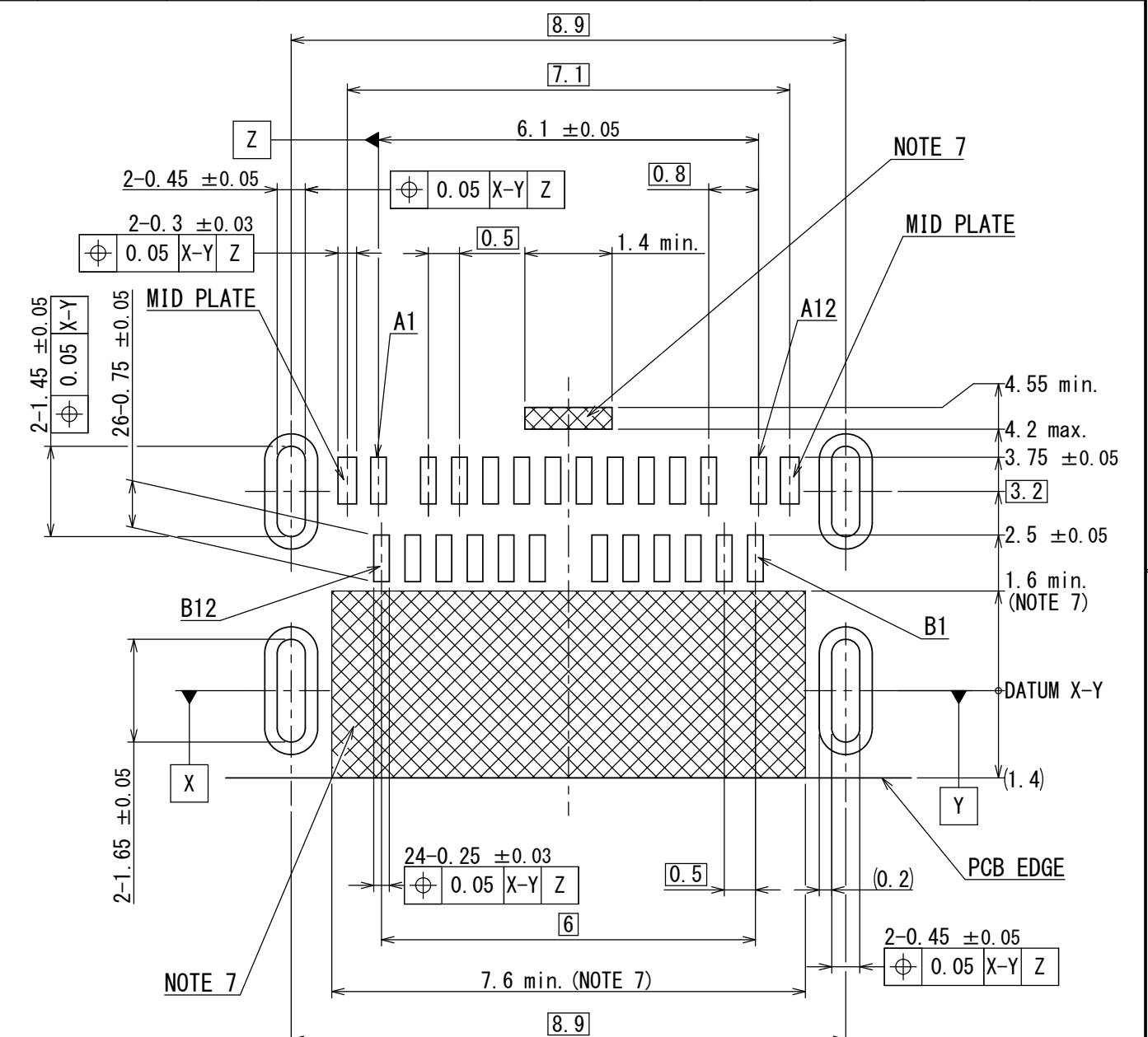
APPLICABLE P.C.B DIMENSION (REF.) (10 : 1)
