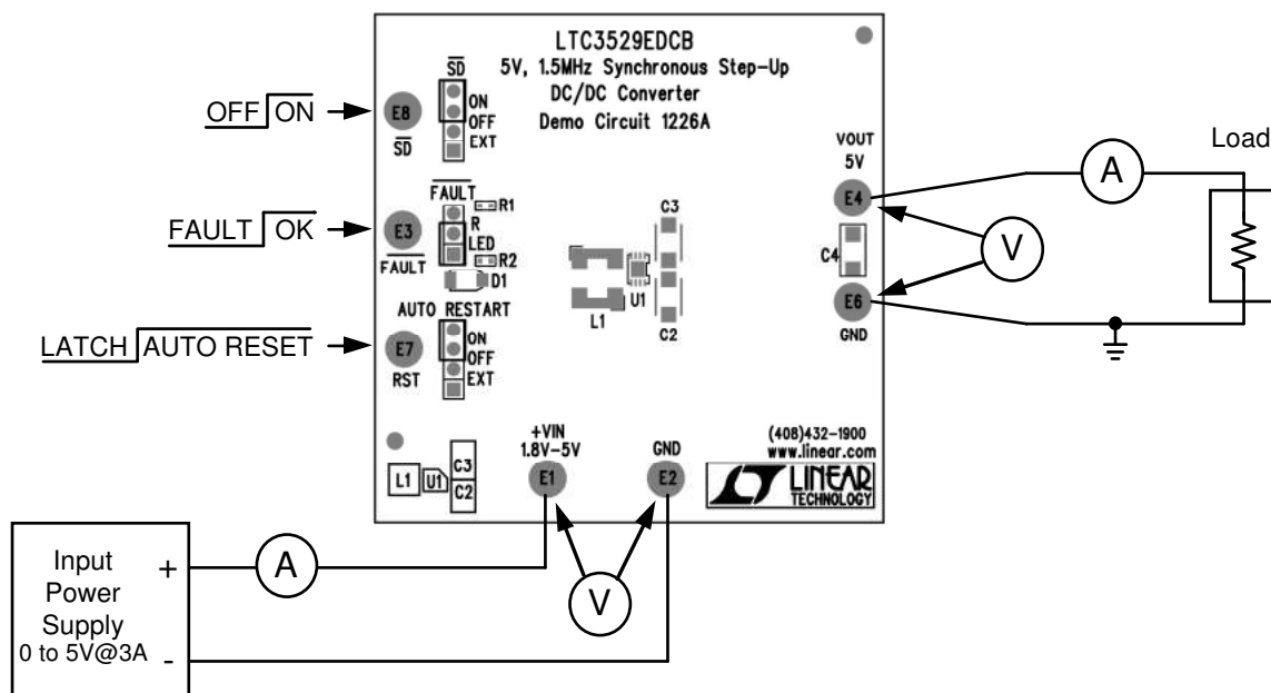
Figure 1. Demonstration Circuit Test Setup
