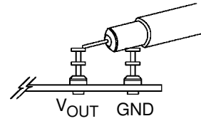
Figure 4. Scope Probe Placement for Measuring Output Ripple Voltage
