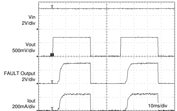
Figure 2. Auto Restart Overload Fault Detection Waveforms For a 3Ω Load.
