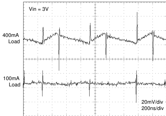
Figure 3. Typical Output Ripple Voltage
