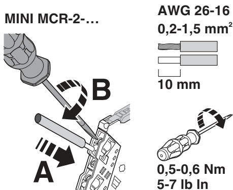
Figure 4 Screw connection
