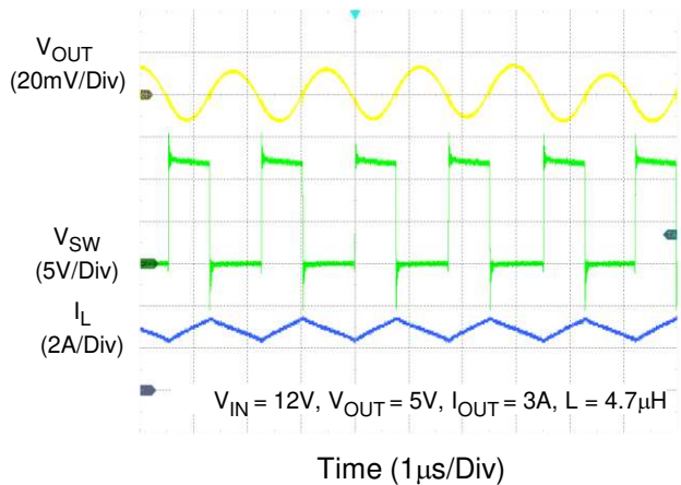
Output Ripple as IOUT = 3A
