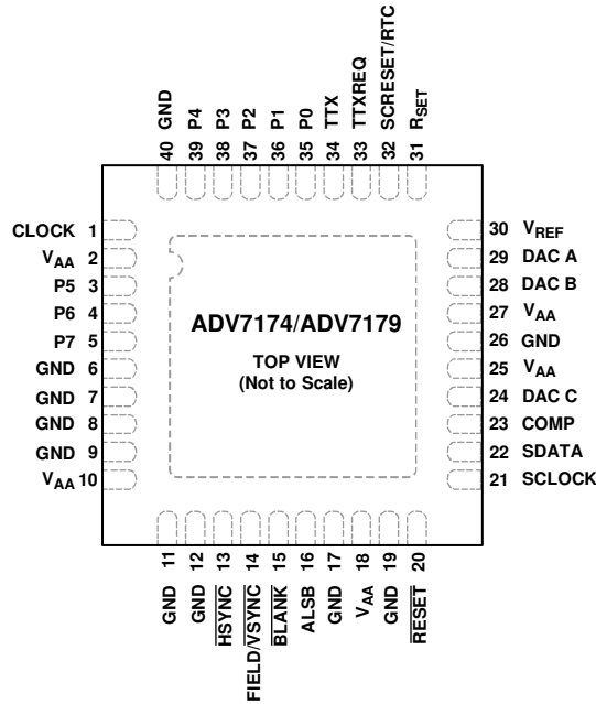
Figure 5. Pin Configurations
