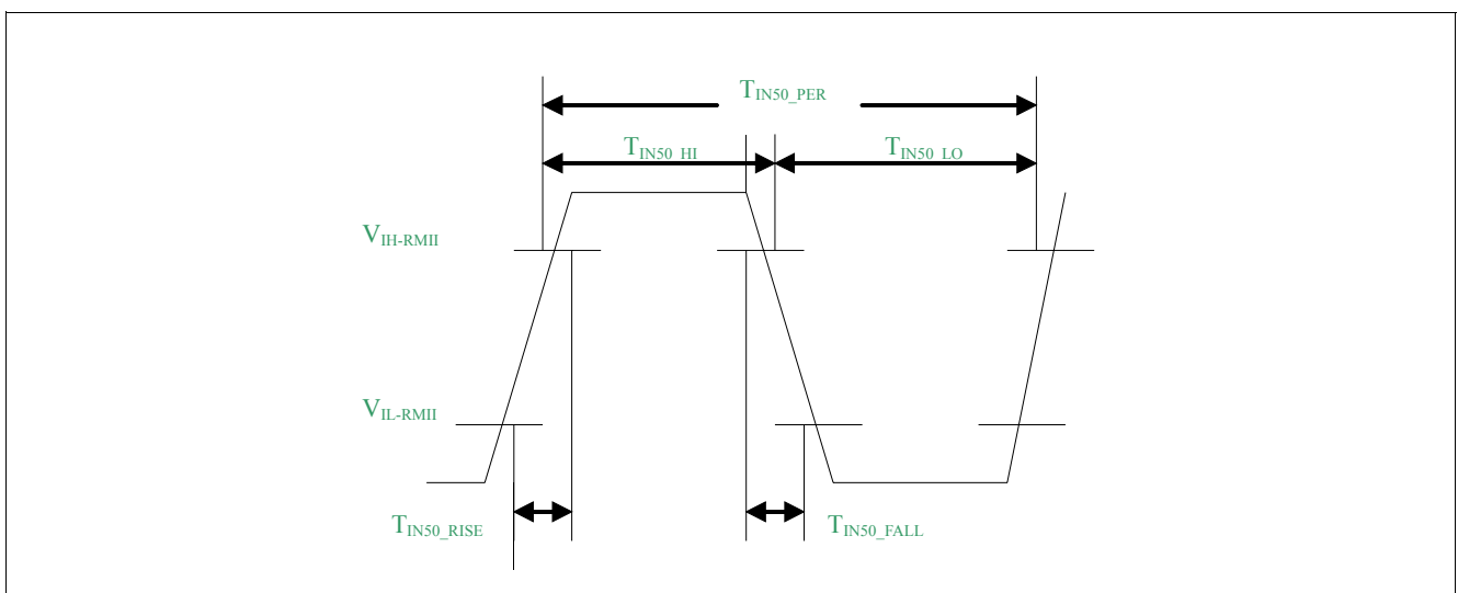
Figure 26 RMII REFCLK Input Timing
