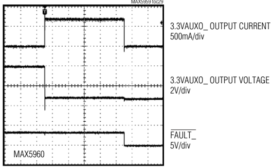
SHORT CIRCUIT ON 3.3AUXO - (AUXILIARY OUTPUT)
