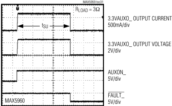
POWER-UP INTO FAULT (AUXILIARY SUPPLY)
