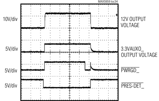
PRESENT-DETECT (ON/OFF) OPERATION
