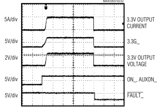
POWER-UP INTO FAULT (3.3V MAIN)
