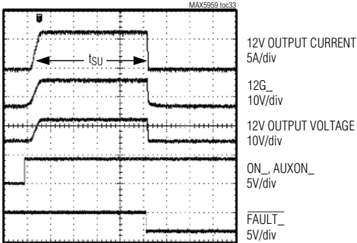
POWER-UP INTO FAULT (12V MAIN OUTPUT)
