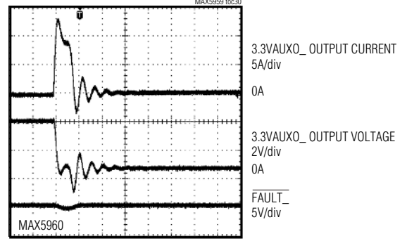
SHORT CIRCUIT ON 3.3VAUXO - (AUXILIARY OUTPUT)
