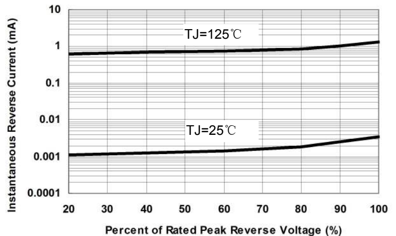
Fig.2-Typical Reverse Characteristics
