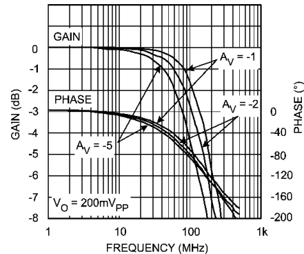
Figure 2. Inverting Frequency Response
