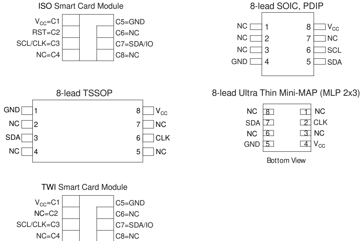
Figure 1. Pin Configuration
