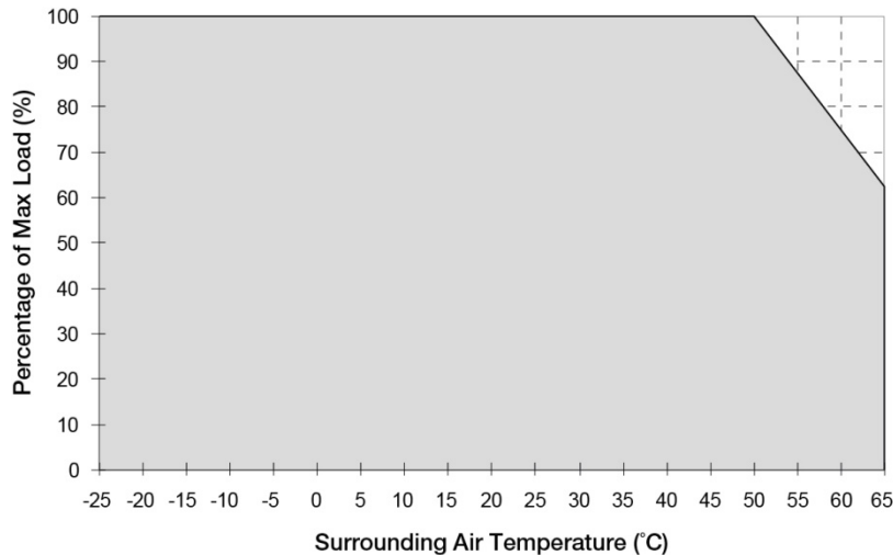
Fig. 1 De-rating for Vertical Mounting Orientation > 50°C de-rate power by 2.5% / °C
