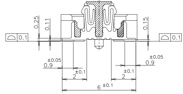
F-F (GROUND POSITION) (SCALE 8:1)
