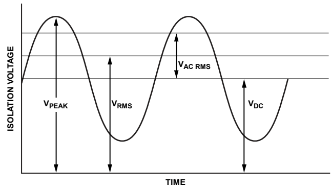
Figure 45. Critical Voltage Example
