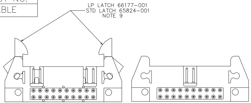
HEADER WITH LATCHES
