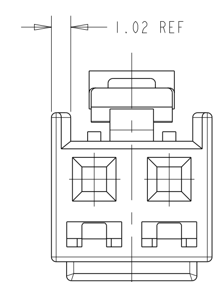
FRONT VIEW (2 POSITION SHOWN)
