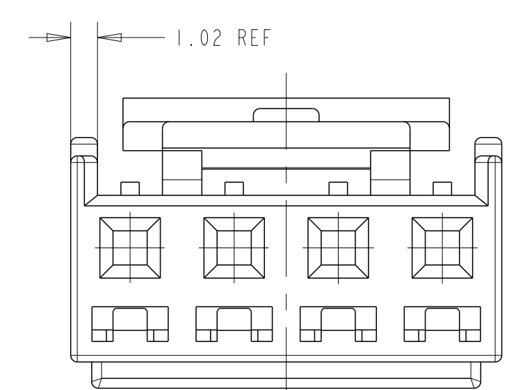
FRONT VIEW (4 POSITION SHOWN)
