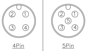
Pin Assignments Front View
