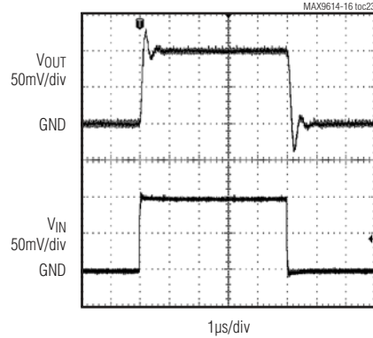
100mV STEP RESPONSE C LOAD = 200pF
