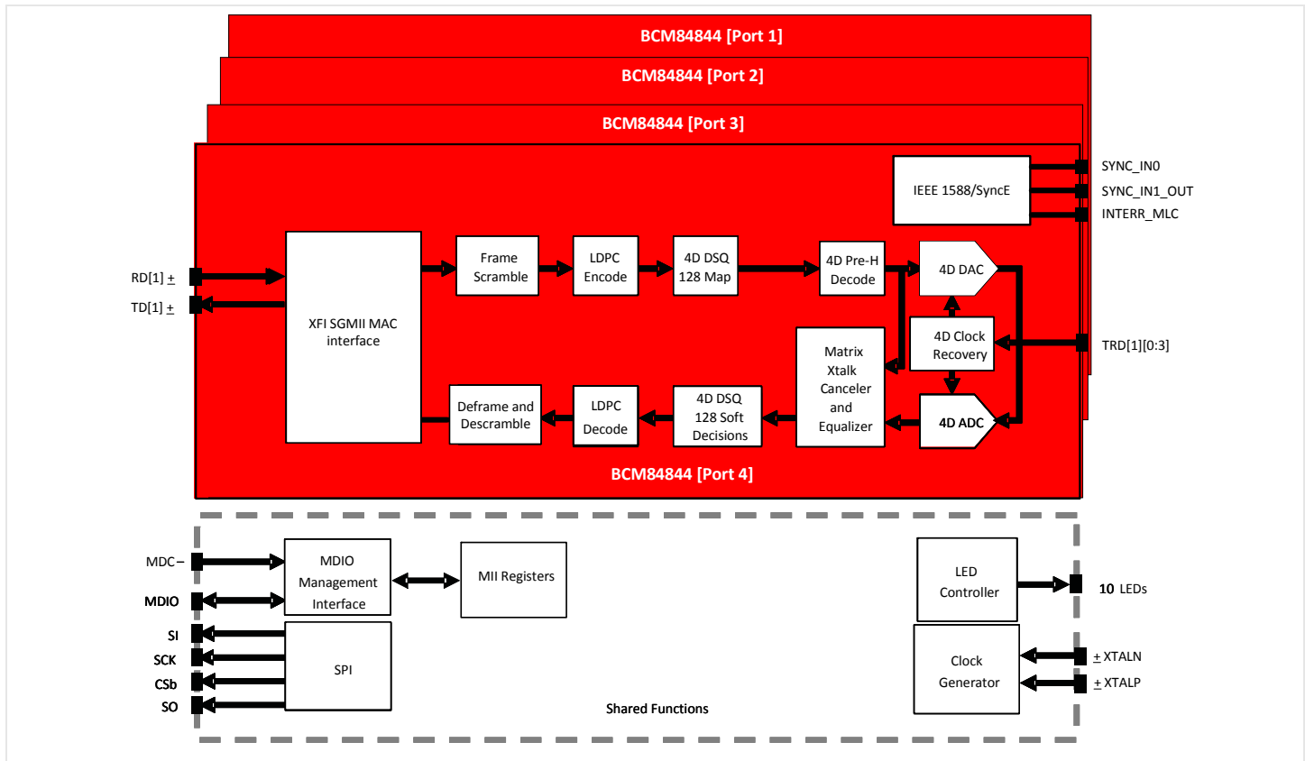
BCM84844 Block Diagram for Each Port
