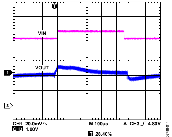
Figure 36. LDO Response to Line Transient, Input Voltage from 4.5 V to 5 V, V_{OUT3} = 2.8\text{ V}
