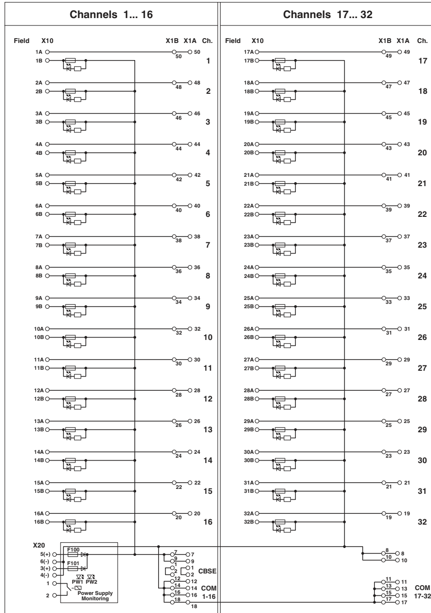
Circuit diagram
