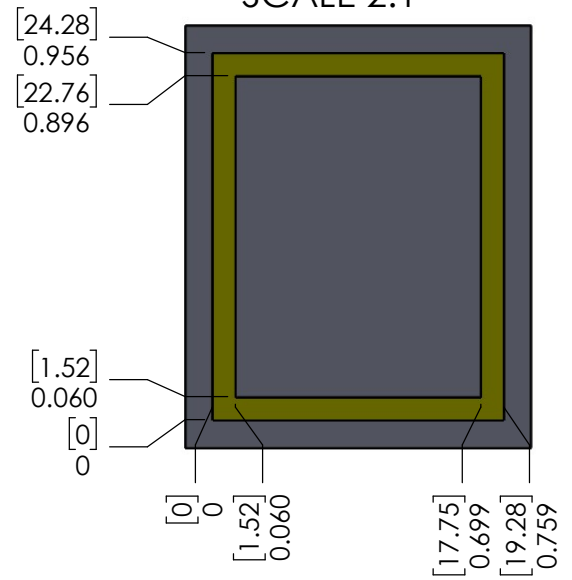
TRACE PATTERN SCALE 2:1
