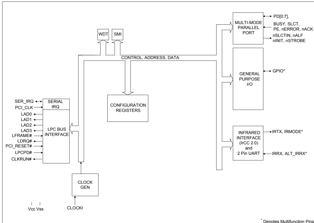
Figure 1 SIO1036 Block Diagram
