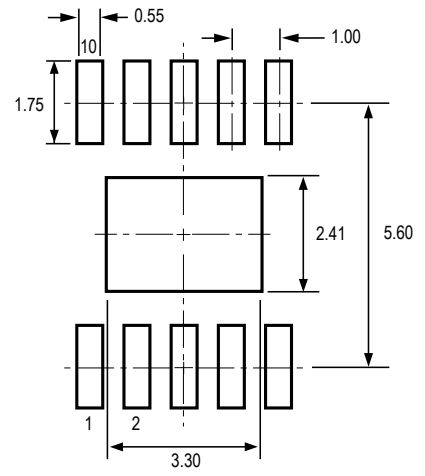
△ C PCB Layout Reference View
