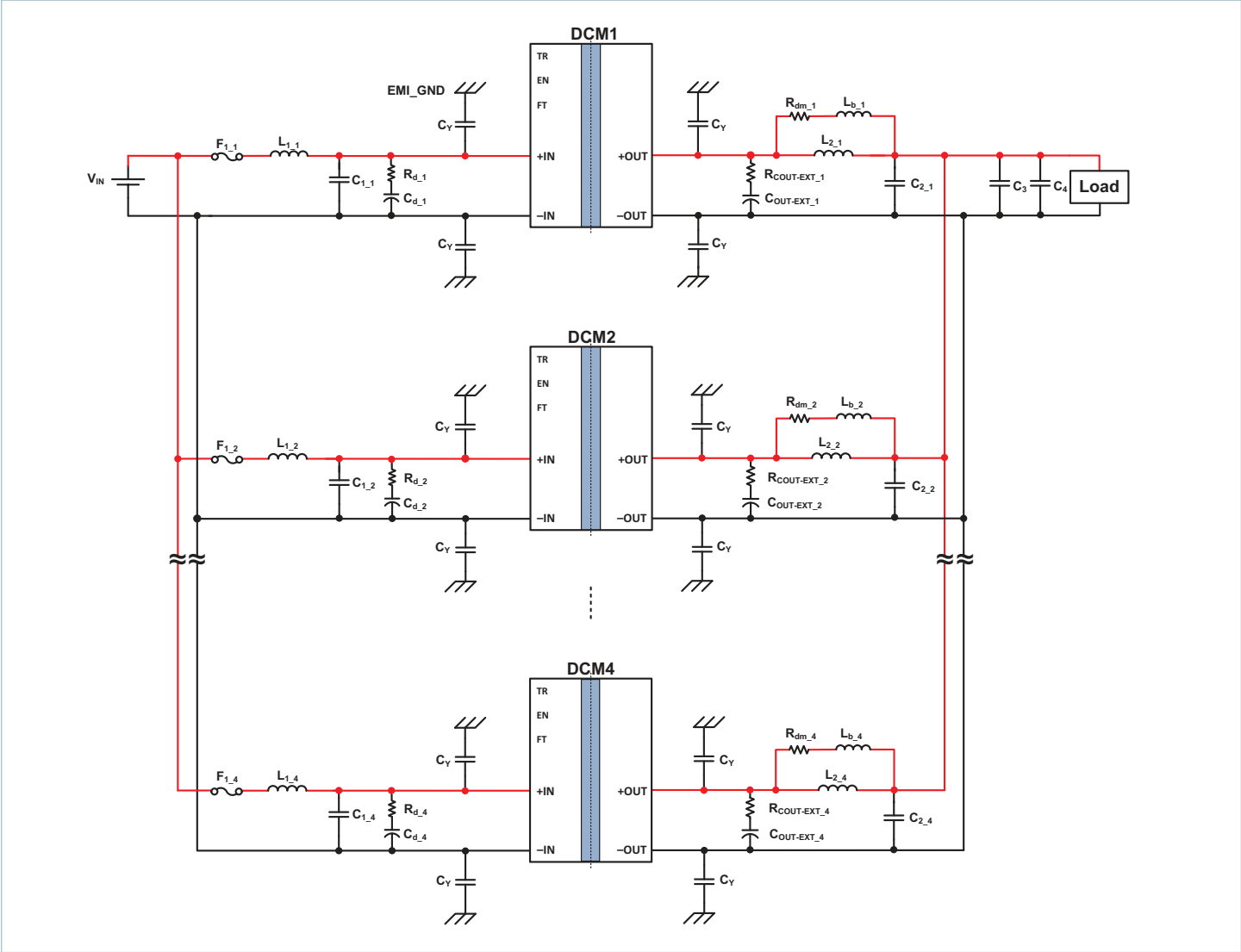
Typical Application 1: DCM4623xD2K13E0yzz in an array of four units
