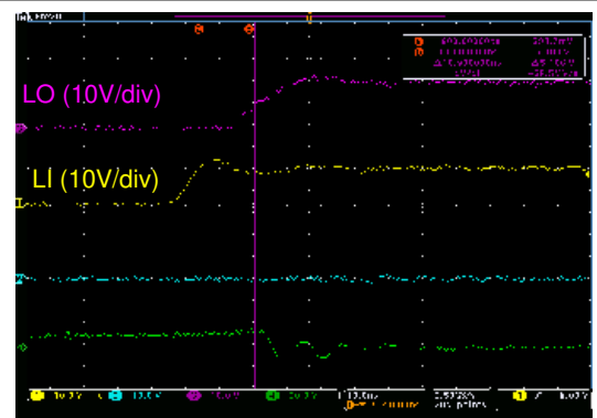
Figure 8-7. Turn-on Propagation Delay
