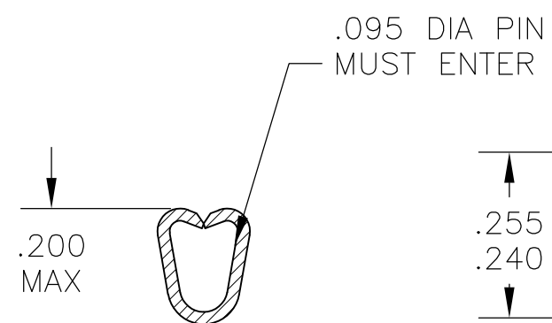
SECT B-B PRE-CRIMP WITH .140 F CRIMPER
