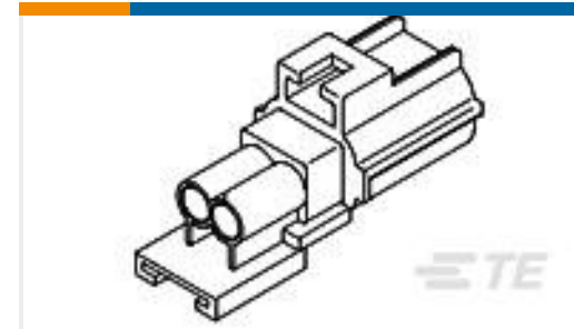
TE Part #184153-1 2 POS. END CAP HSG., KEY C
