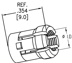
CABLE COLLET
