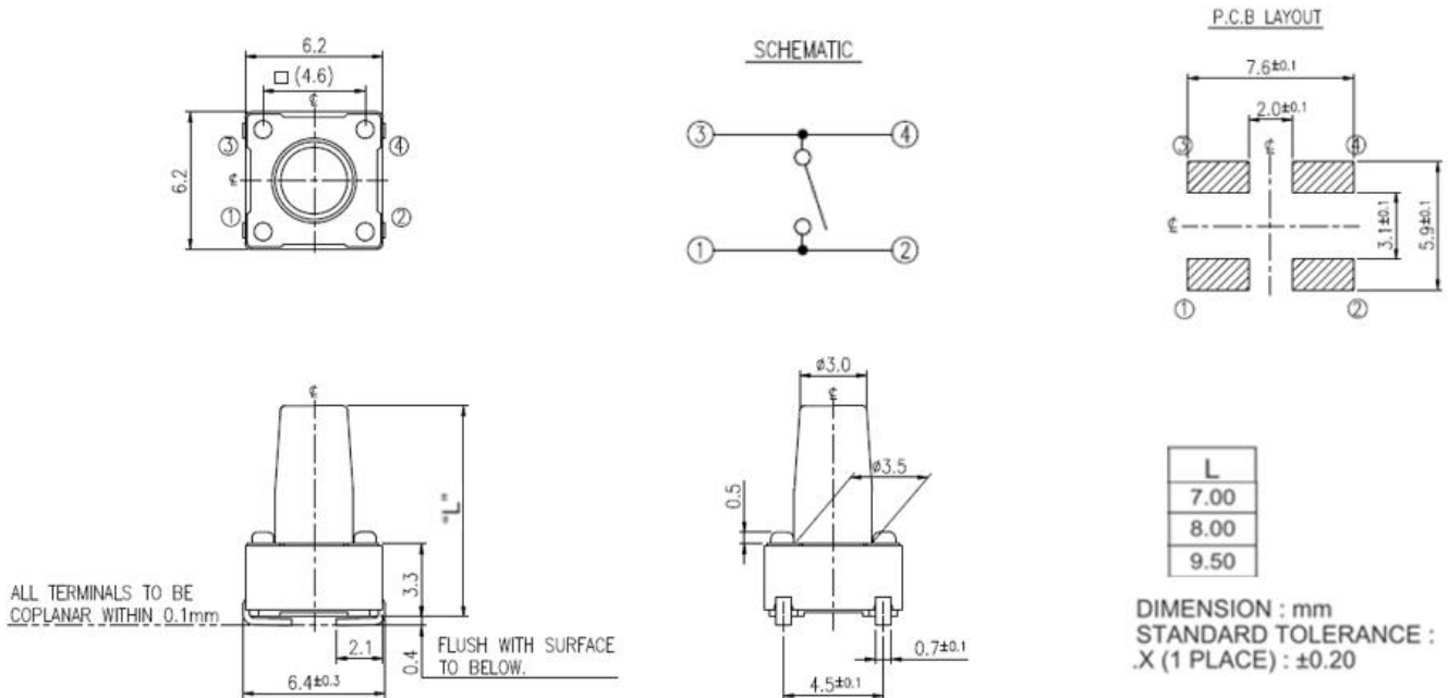
Figure 5 – Surface Mount U terminal type, 222AU, Vertical Actuation
