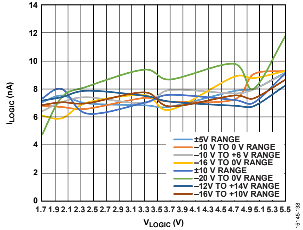
Figure 55. Logic Current ( I_{Logic} ) vs. Logic Input Voltage ( V_{Logic} )
