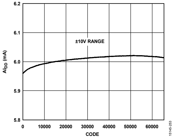
Figure 53. Supply Current ( I_{bD} ) vs. Code
