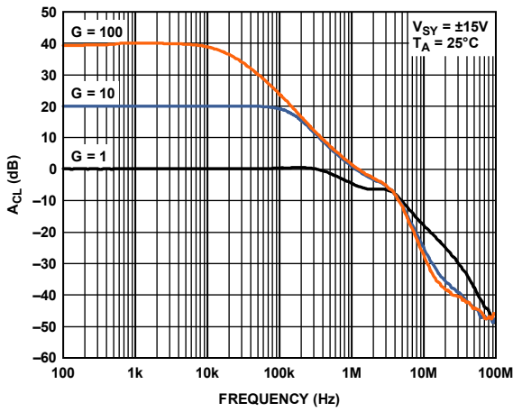
Figure 30. Closed-Loop Gain vs. Frequency
