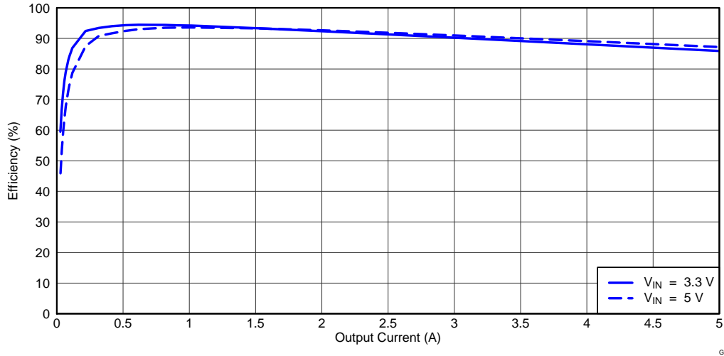
Figure 1. TPS54519EVM-037 Efficiency
