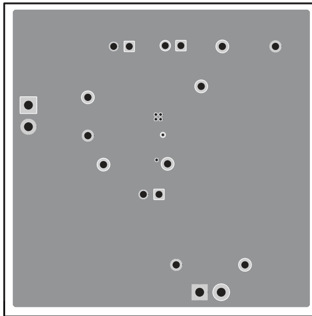
Figure 15. TPS54519EVM-037 Layout 2
